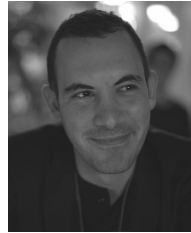
formal verification.
